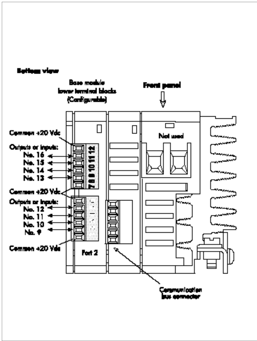
Figure 2-2 Base module control terminal identification (lower terminal blocks)
