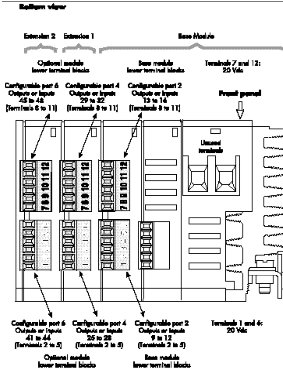
Figure 2-4 Control terminal block identification (2 extension modules, lower terminal blocks)
