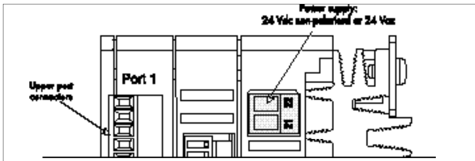
Figure 2-7 REMIO power supply terminal (seen from above)
