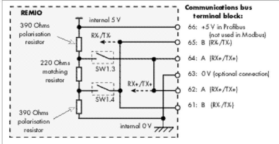
Figure 4-2 Termination resistor configuration (Modbus and Profibus)
