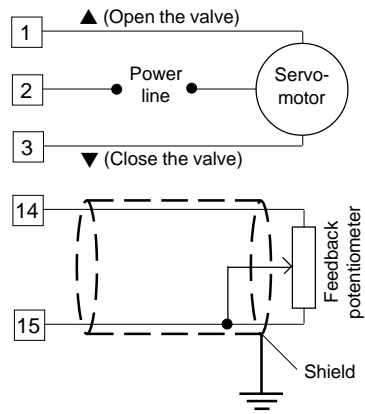
Fig. 8 - SERVOMOTOR WIRING The two relay outputs are interlocked.
