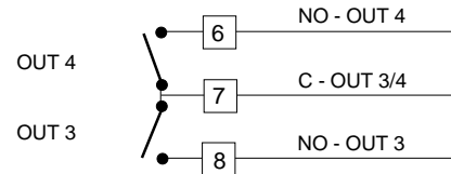
Fig. 9 RELAY OUTPUTS WIRING
