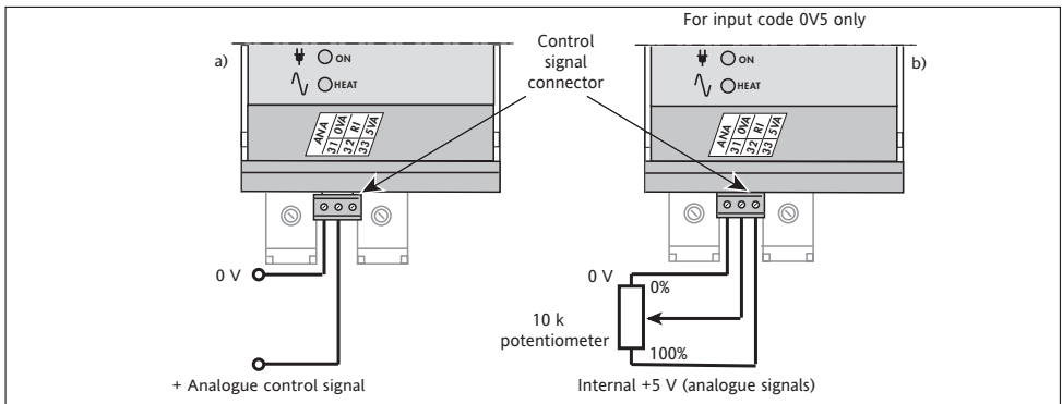
Figure 2-8 Control signal connection (self-powered unit without alarms)
