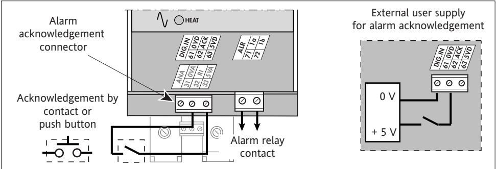
Figure 2-10 Typical alarm relay contact and external acknowledgement connections
