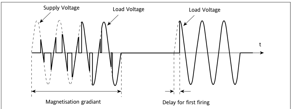
Figure 3-7 Transformer primary power-up in 'Burst mode' (XFMR option)
