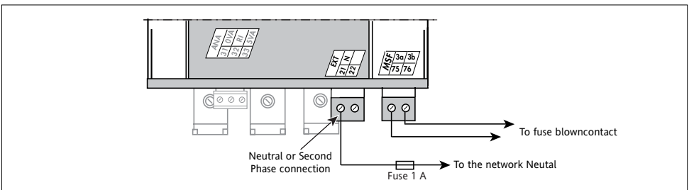
Figure 2-11 Connecting the supply neutral voltage
