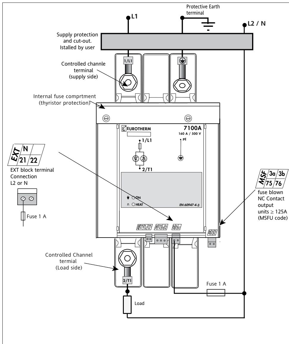
Figure 2-7 7100A power thyristor unit power and input signal connections (rating ≥ 100 A, self-powered electronics)
