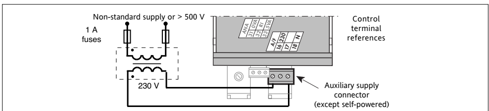
Figure 2-9 Typical 230 V auxiliary power supply connection
