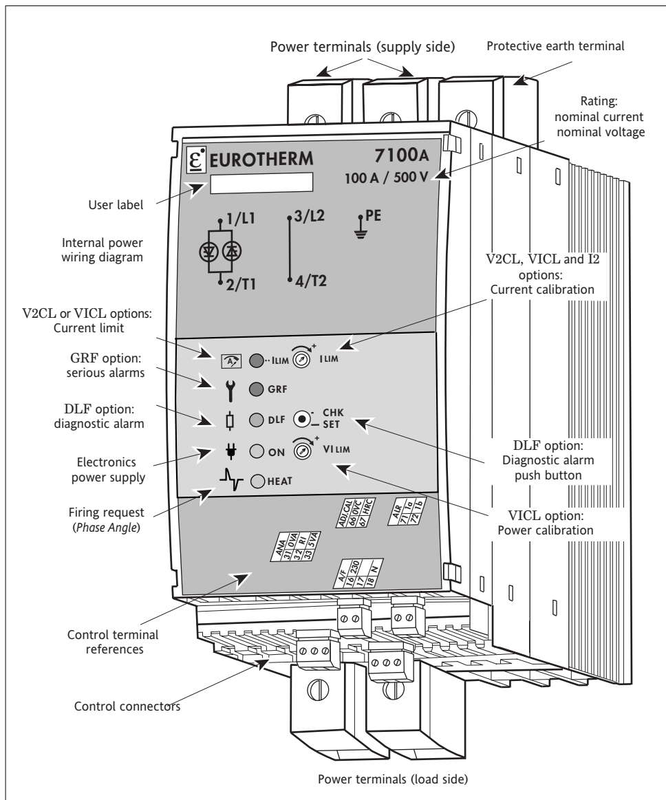
Figure 1-3 General view of 7100A power thyristor unit 80A to 100A 'full' version
