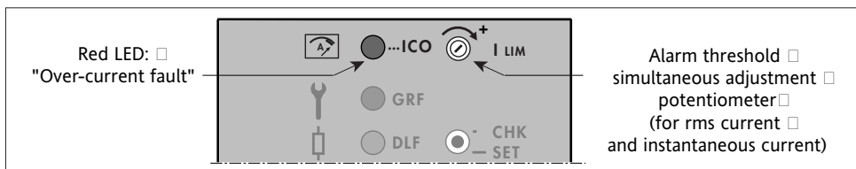
Figure 5-4 Layout of the 'ICO' LED and 'I lim' potentiometer with the ICO option
