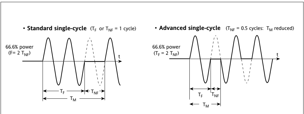
Figure 3-4 Example of Single-cycle and Advanced single-cycle firing mode
